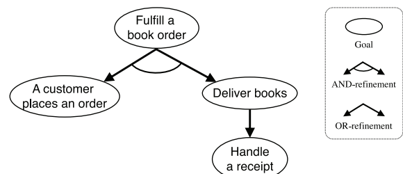
Fig. 1 Example goal graph having poor refinement.
