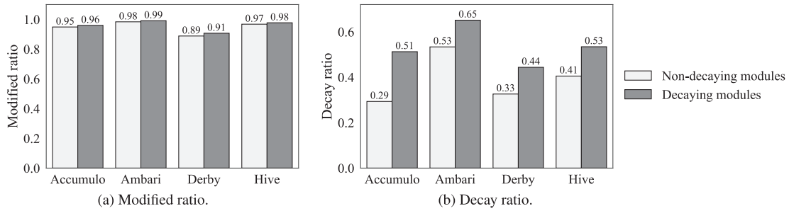
Fig. 4 Averages of the number of decaying and non-decaying classes that will be modified and decay.
