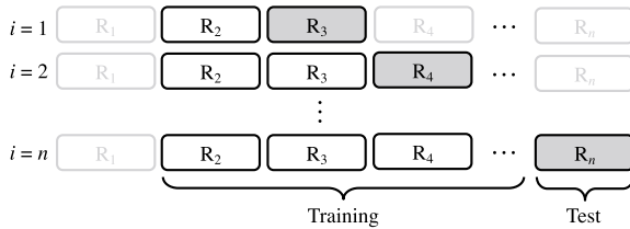
Fig. 6 Training and test data separation.
