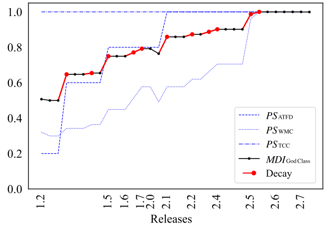
Fig. 2 The decaying process of AmbariServer.
