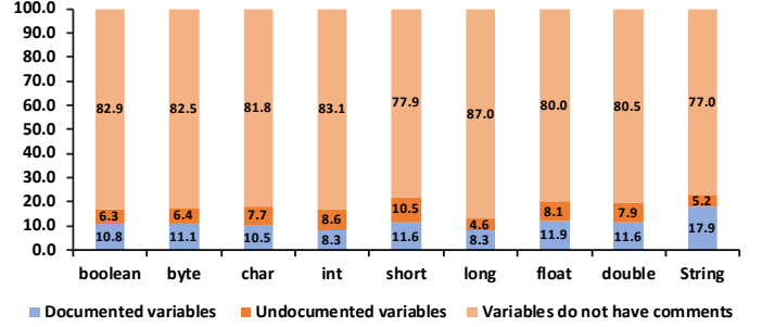
Fig. 2. Percentage of variables documented, undocumented in the comment, and the percentage of the variables that do not have comments.
