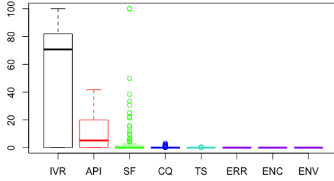
(a) Remained Warnings in RATS
