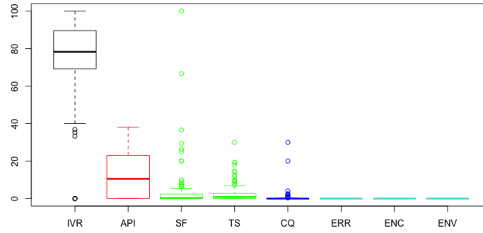
(b) Bug warning categories in RATS at 2017
