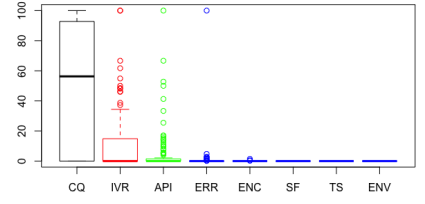
(f) Disappeared Warnings in the PVS-Studio
