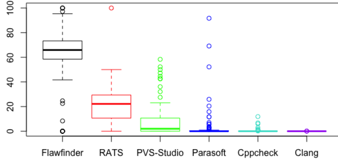
(a) IVR warnings among SAST tools in 2012
