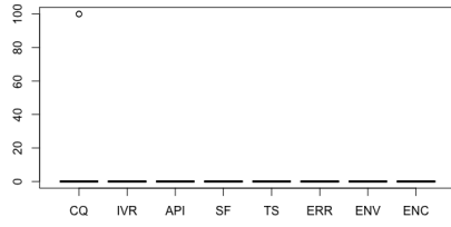
(a) Remained Warnings in the Clang Static Analyzer
