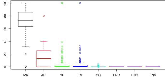
(a) Bug warning categories in RATS at 2012
