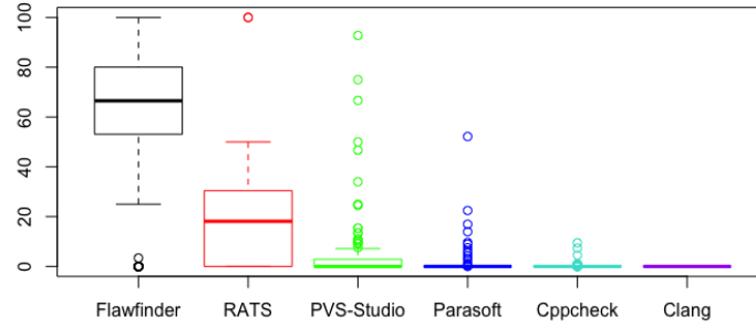
(a) Remained Warnings among IVR
