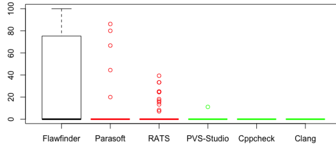
(b) Modified Warnings among IVR
