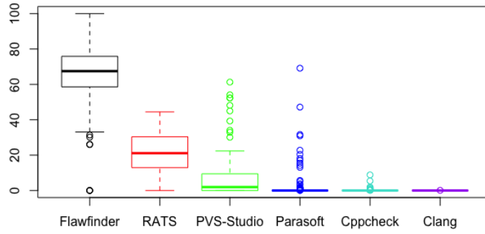
(b) IVR warnings among SAST tools in 2017
