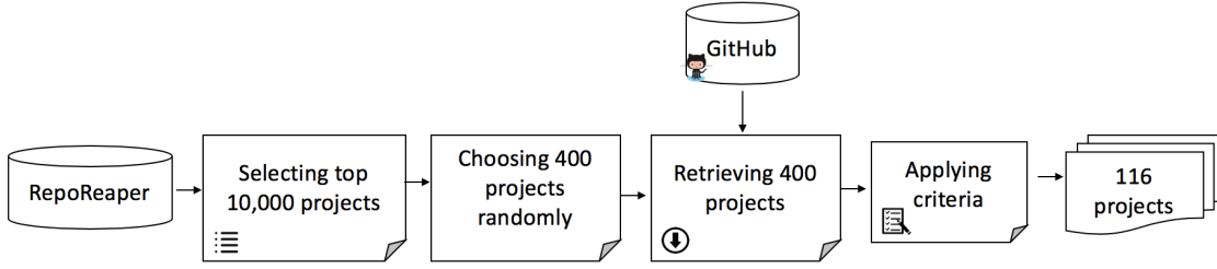
Fig. 1: Case study project selection
