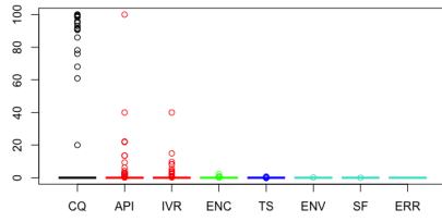
(g) Remained Warnings in the Parasoft C/C++ test
