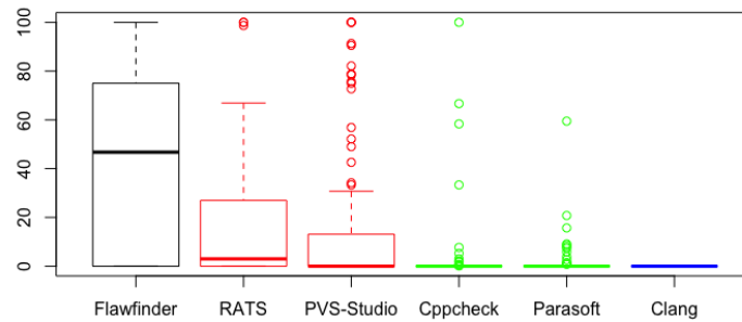
(c) Disappeared Warnings among IVR
