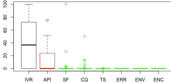
(c) Disappeared Warnings in RATS
