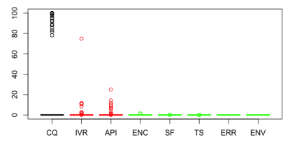
(i) Disappeared Warnings in the Parasoft C/C++ test
