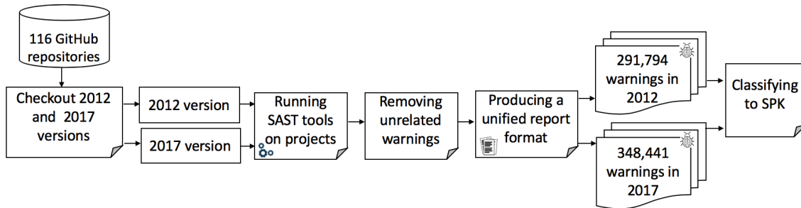
Fig. 3: Extracting security warnings
